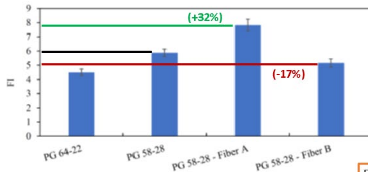
Figure B.14 FI Values for Lab Compacted Samples for Fayette County Mixes
