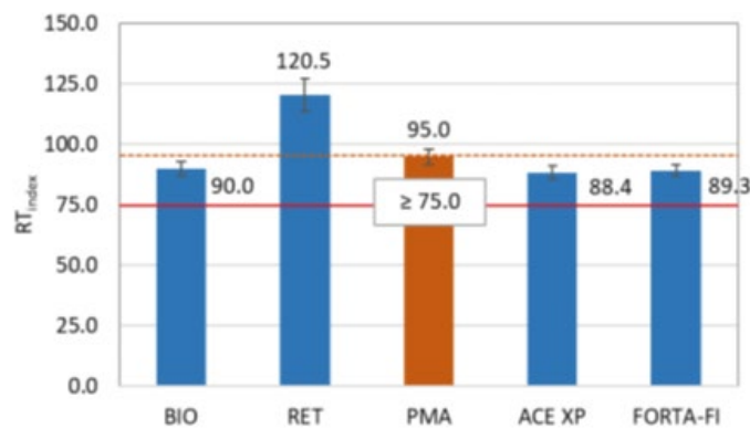
Figure 4-7. IDEAL-RT Tests: (b) RT index at 50.0°C
