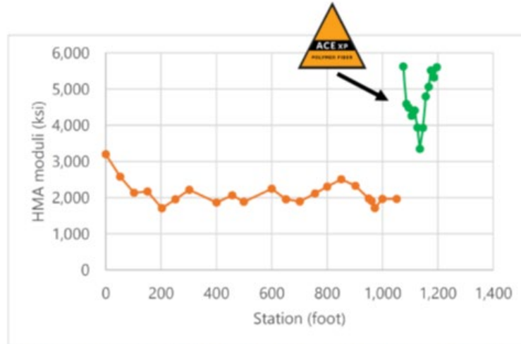
Figure 2-2: Backcalculated HMA moduli for SB Orange and Green sections.
